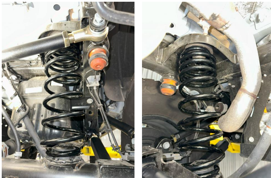
Figure 25: Axle drooped with old springs removed, and bump stops installed
